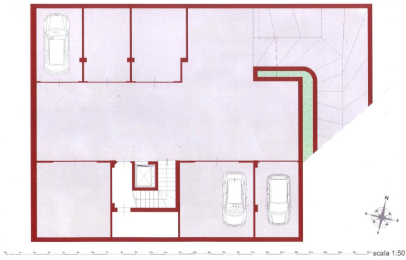
PIANO INTERRATO
